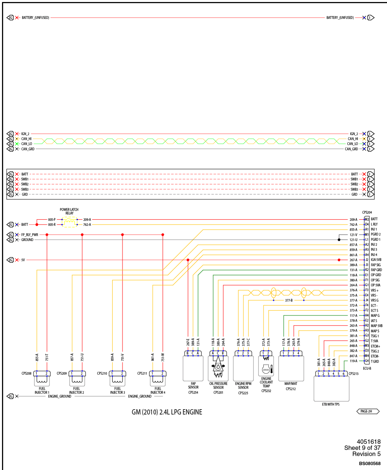
Figure 5. GM (2010) 2.4L LPG Engine Electrical Schematic (Sheet 2 of 2)
