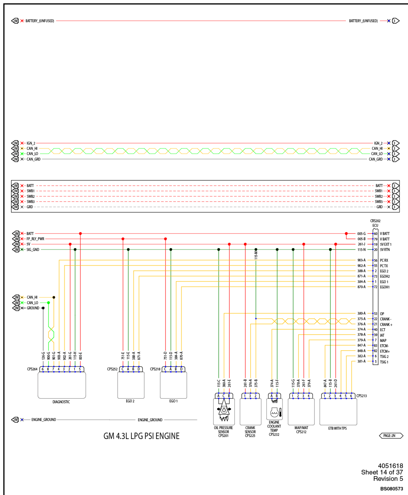
Figure 8. GM 4.3L LPG PSI Engine Electrical Schematic (Sheet 2 of 2)
