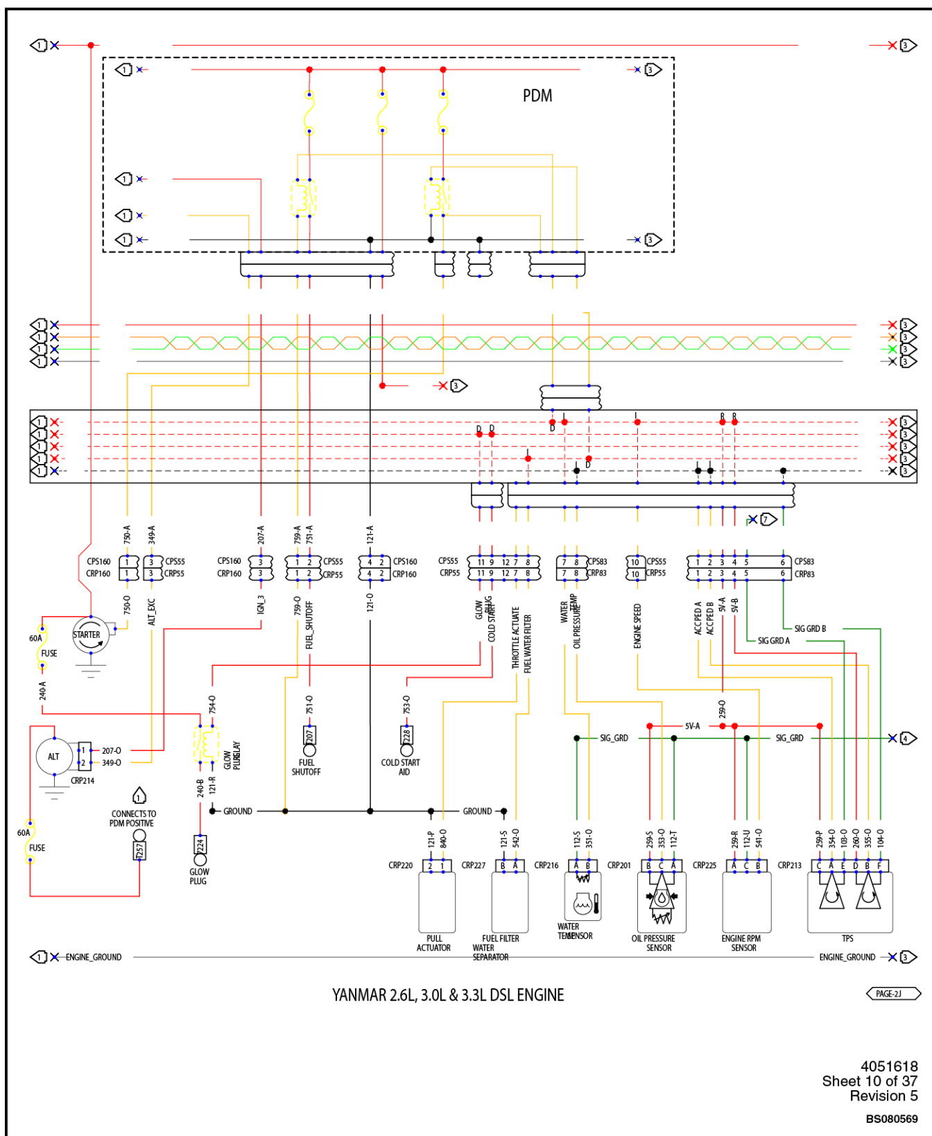
Figure 6. Yanmar 2.6L, 3.0L, and 3.3L Diesel Engine Electrical Schematic
