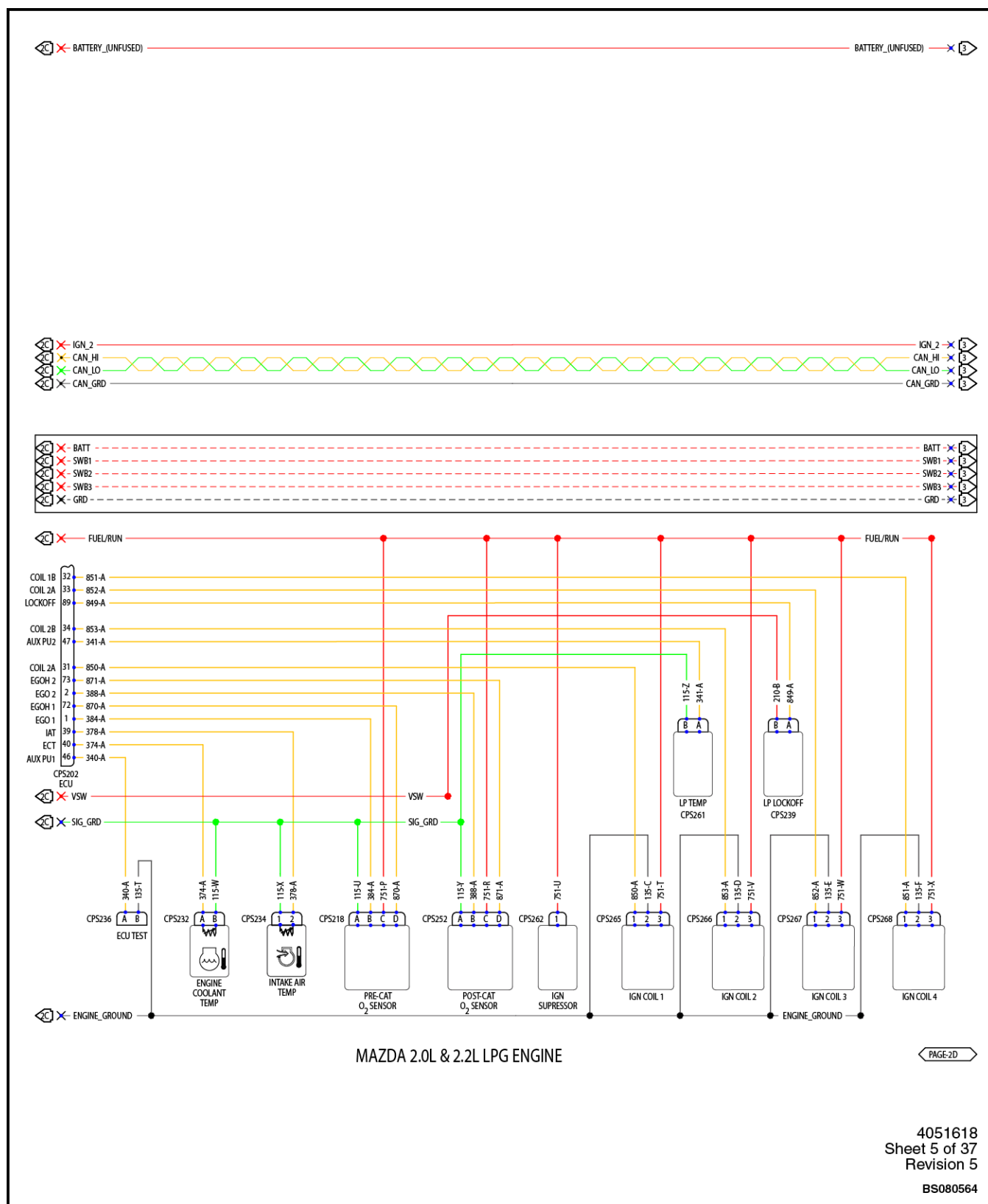
Figure 3. Mazda 2.0L and 2.2L LPG Engine Electrical Schematic (Sheet 2 of 2)
