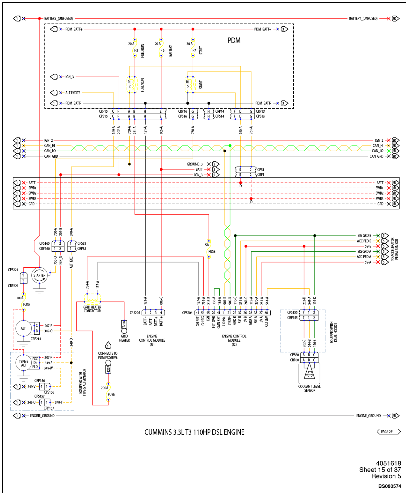
Figure 9. Cummins 3.3L T3 110HP Diesel Engine Electrical Schematic (Sheet 1 of 2)
