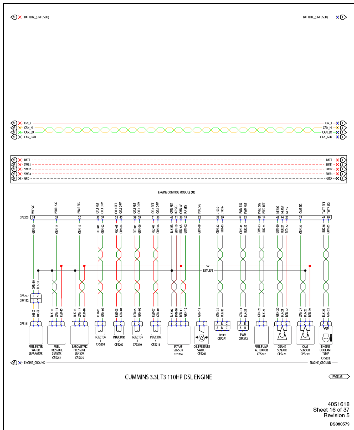
Figure 9. Cummins 3.3L T3 110HP Diesel Engine Electrical Schematic (Sheet 2 of 2)
