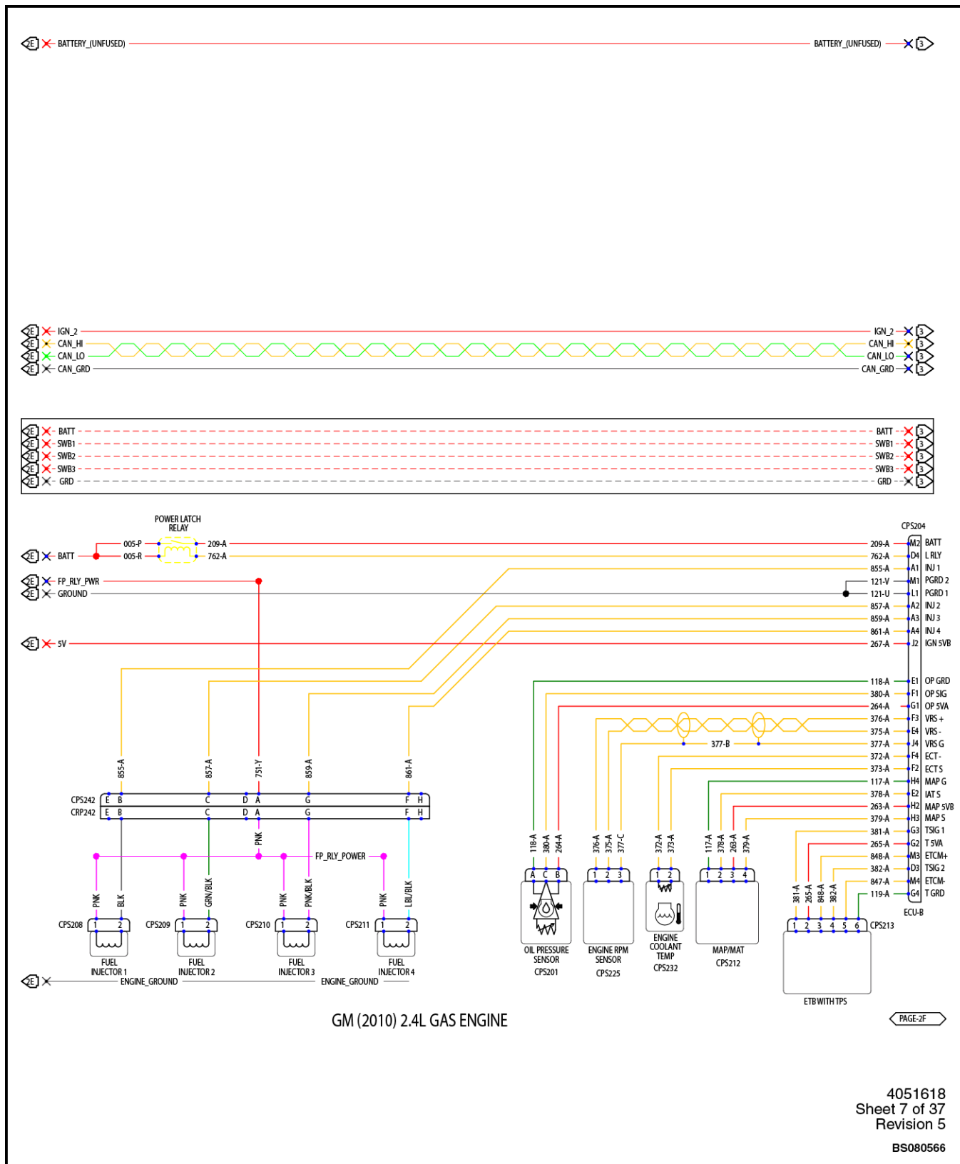
Figure 4. GM (2010) 2.4L Gas Engine Electrical Schematic (Sheet 2 of 2)
