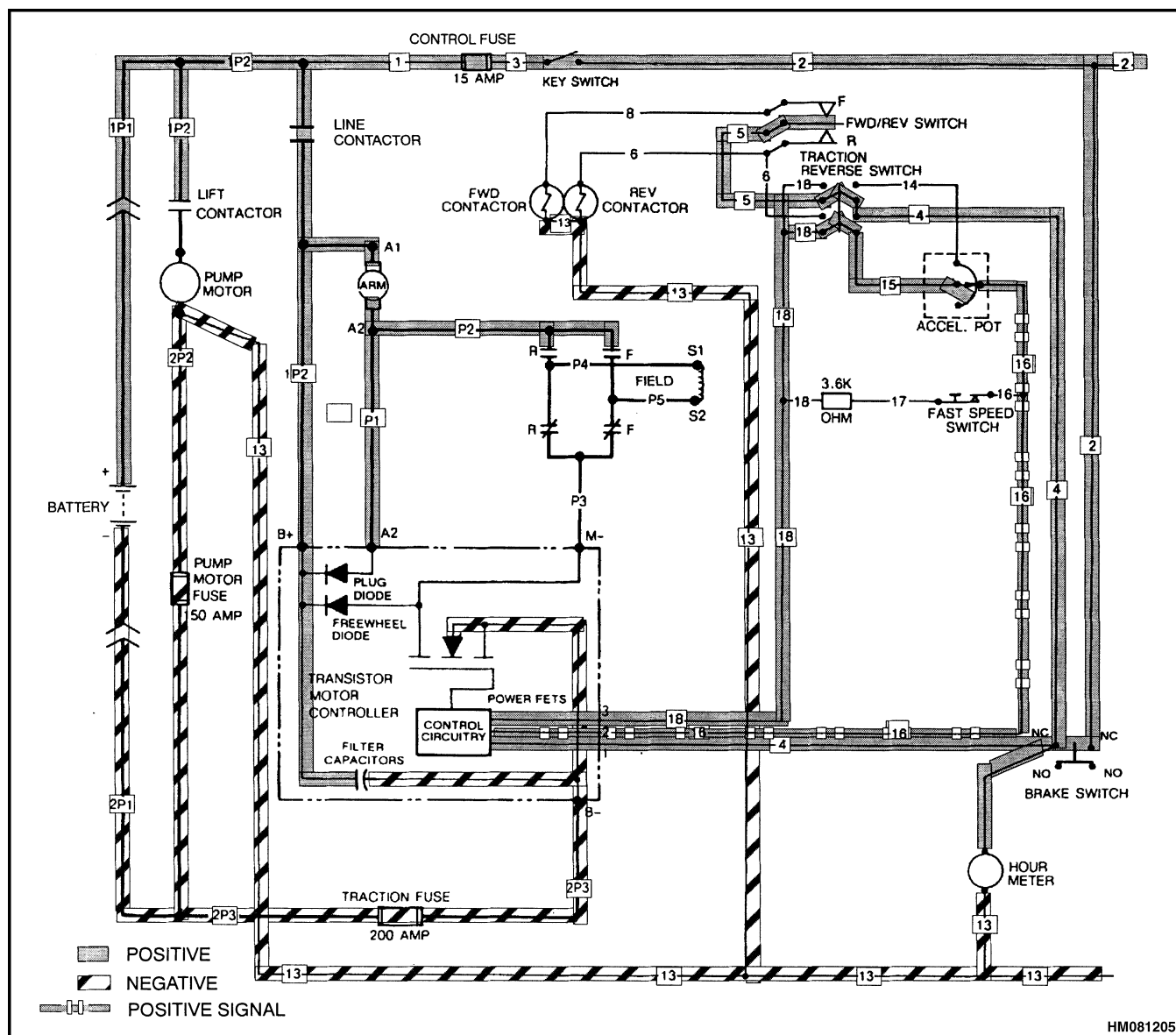
Figure 16. Sequence of Operation - Direction/Speed Control Set for Slow Forward Speed
