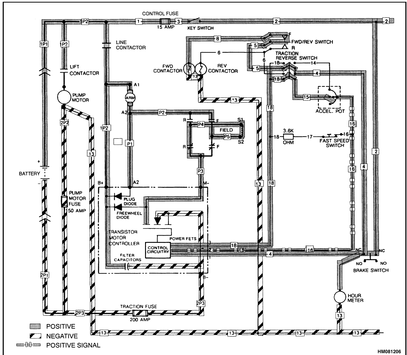
Figure 17. Sequence of Operation - Forward Contactor Energized
