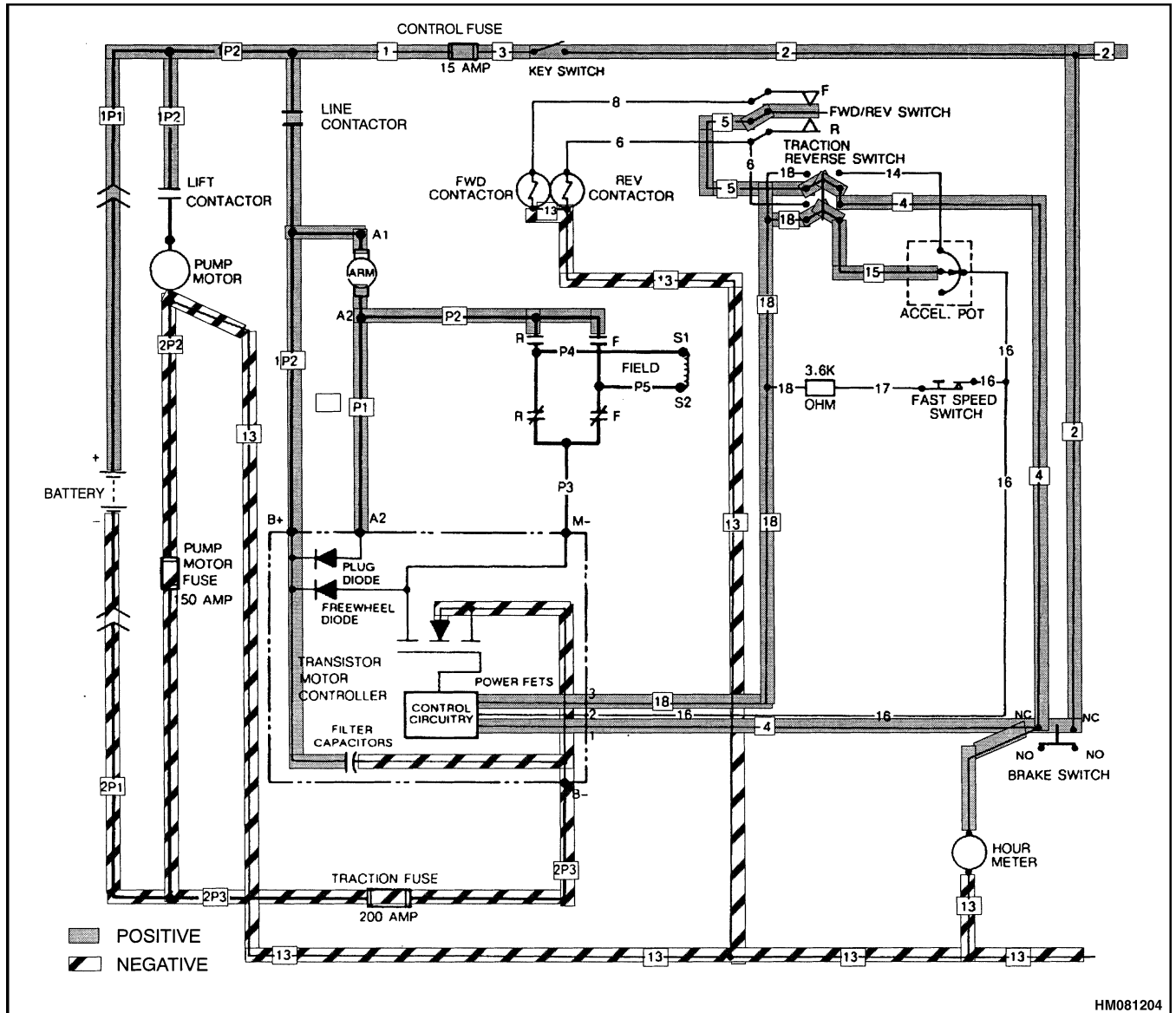
Figure 15. Sequence of Operation - Power to Control Circuit
